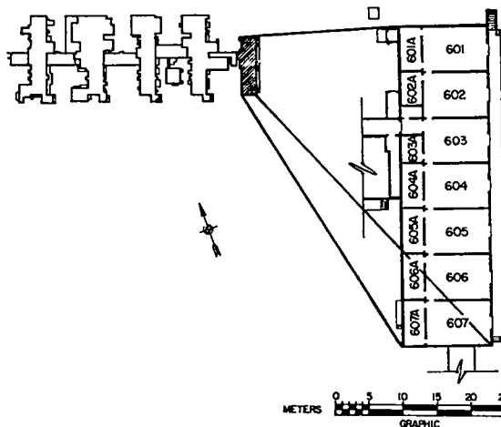
Fig. 10. Floor plan of Building 150.
