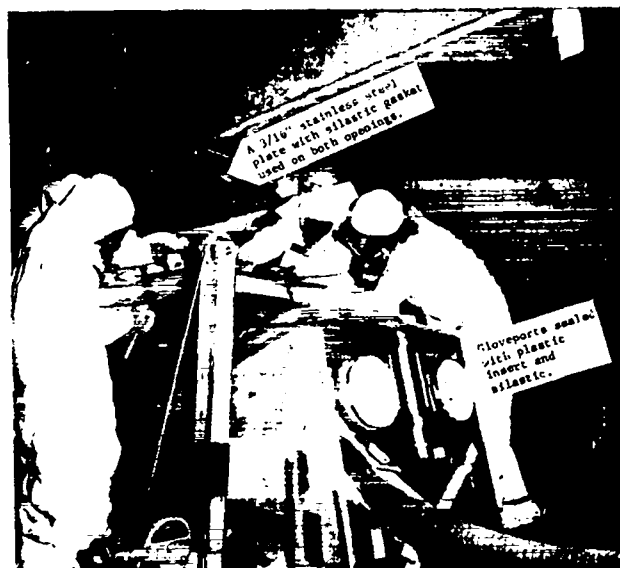
Fig. 8. Glovebox-conveyor tunnel separations.
