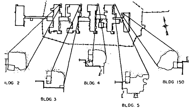
Fig. 36. Location of acid waste sampling wells.
