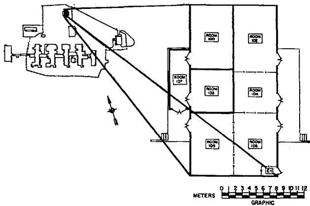
Fig. 35. Floor plan of Building 286.
