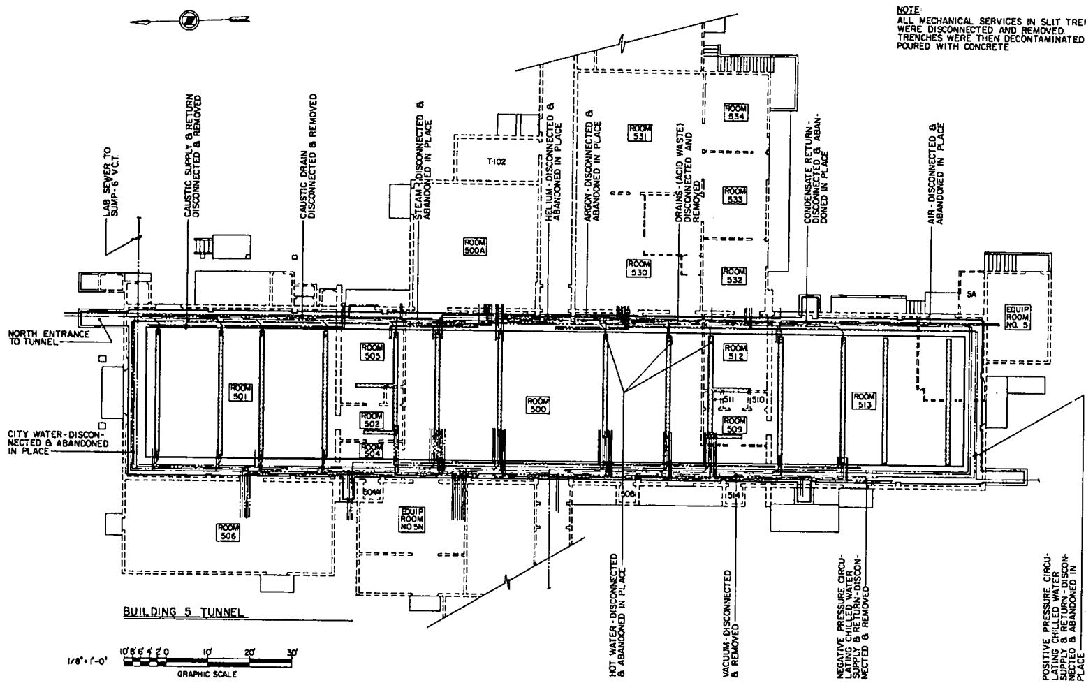
Fig. 19. Utility tunnel around Building 5.
