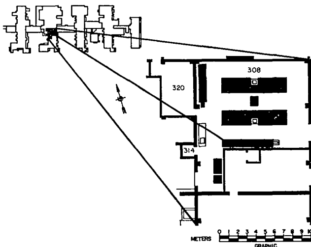
Fig. 30. Floor plan of Room 308 and adjoining support rooms.
