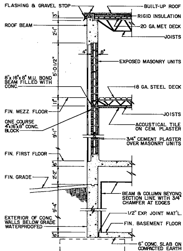
TYPICAL WALL SECTION BUILDING 150
