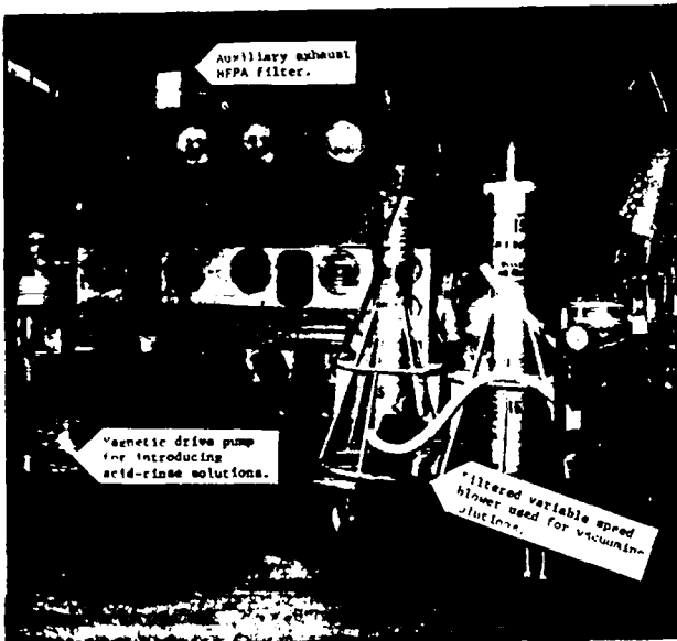
Fig. 7. Glovebox washing and vacuuming apparatus.
