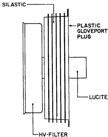
Fig. 44. Gloveport vacuum device.
