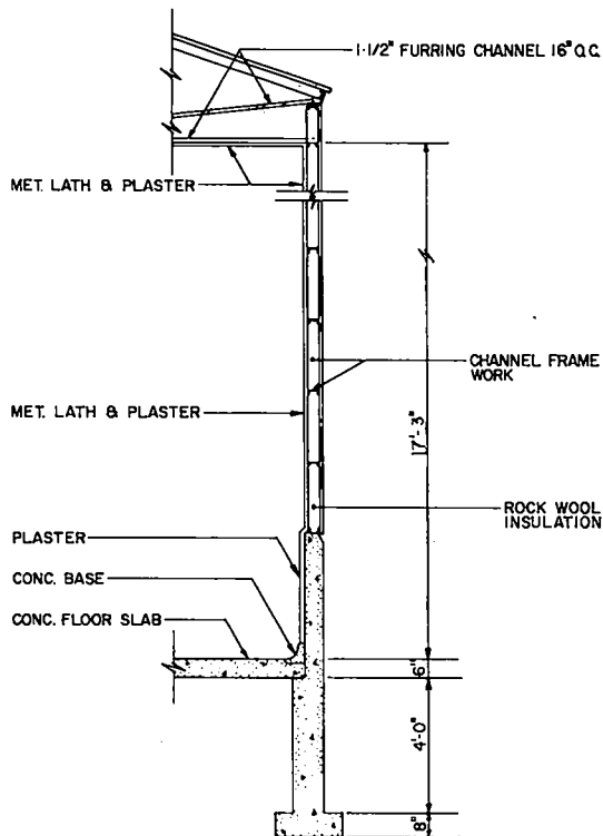
TYPICAL WALL SECTION BUILDINGS 2, 3, 4 & 5
