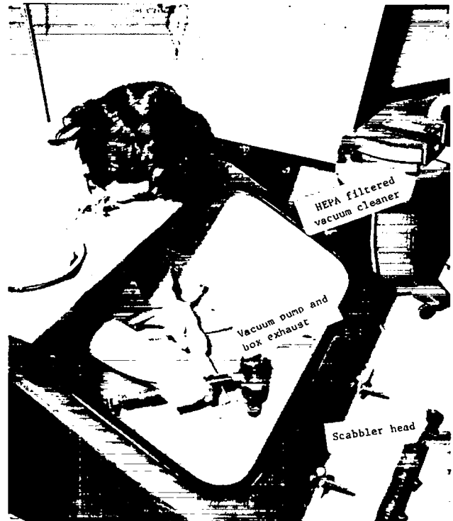
Fig. 46. Confinement chamber for scarifying.
