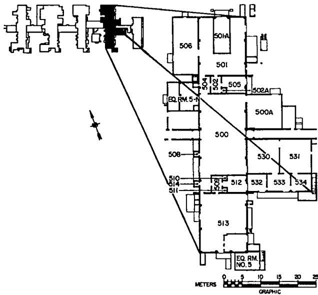
Fig. 17. Floor plan of Building 5.
